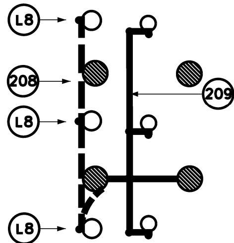
PLAN VIEW OF EARTH CONNECTIONS ON SEALING END PLATFORM
